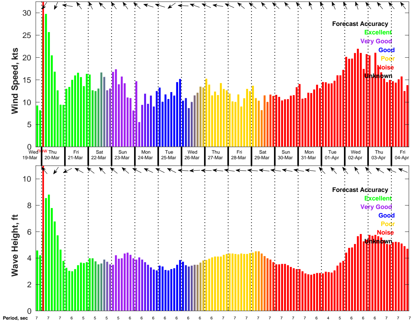
Wind & Wave Forecast for NDBC 42020 from 19-Mar-2025 18:00:00 to 04-Apr-2025 18:00:00
