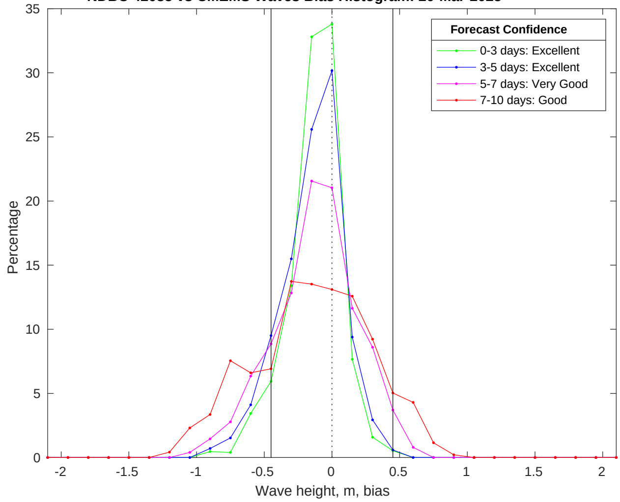
NDBC 42035 vs CMEMS Waves Bias Histogram: 20-Mar-2025
