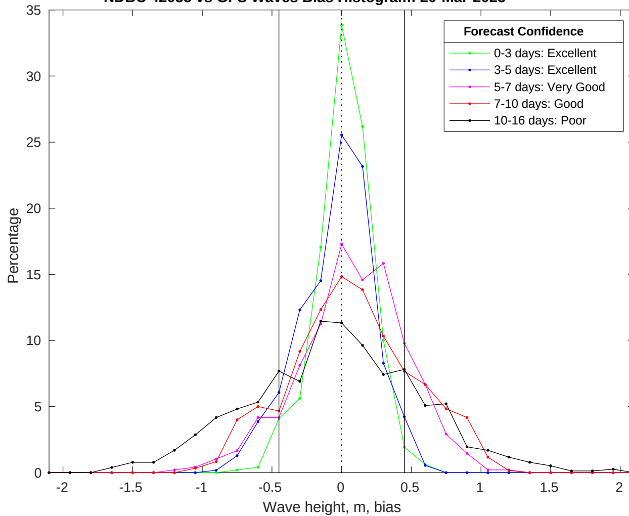
NDBC 42035 vs GFS Waves Bias Histogram: 20-Mar-2025
