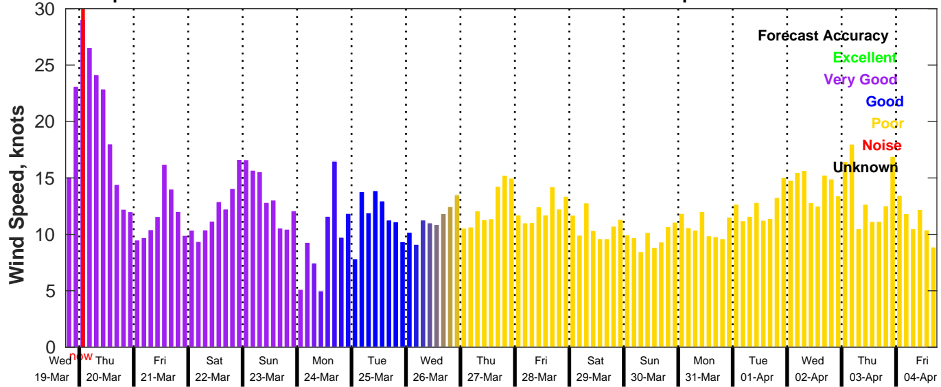
GFS Wind Speed Forecast for NDBC 42035 from 19-Mar-2025 18:00:00 to 04-Apr-2025 18:00:00
