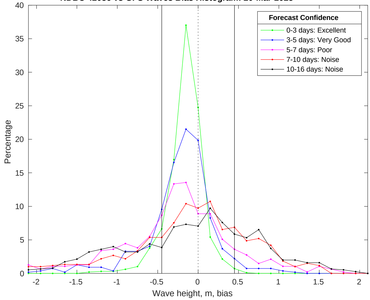
NDBC 42036 vs GFS Waves Bias Histogram: 20-Mar-2025
