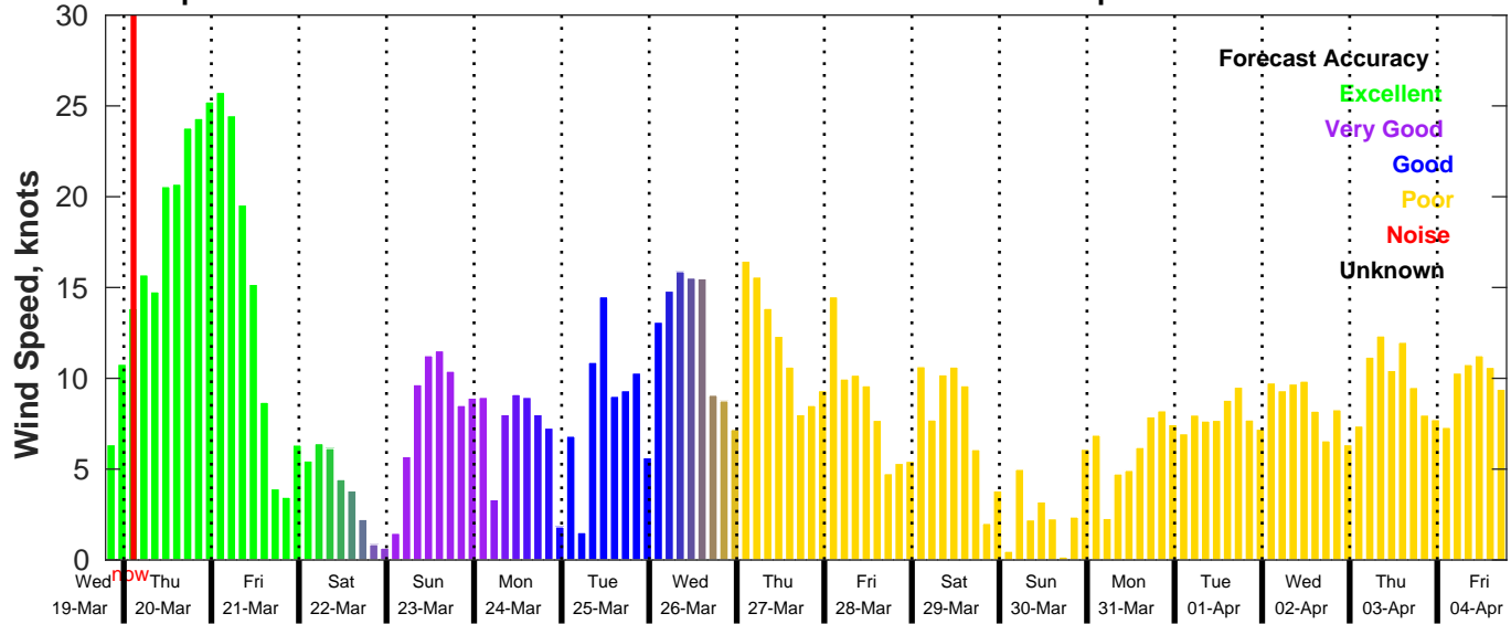
GFS Wind Speed Forecast for NDBC 42036 from 19-Mar-2025 19:00:00 to 04-Apr-2025 19:00:00
