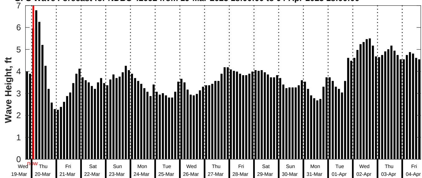
GFS Wave Forecast for NDBC 42092 from 19-Mar-2025 18:00:00 to 04-Apr-2025 18:00:00
