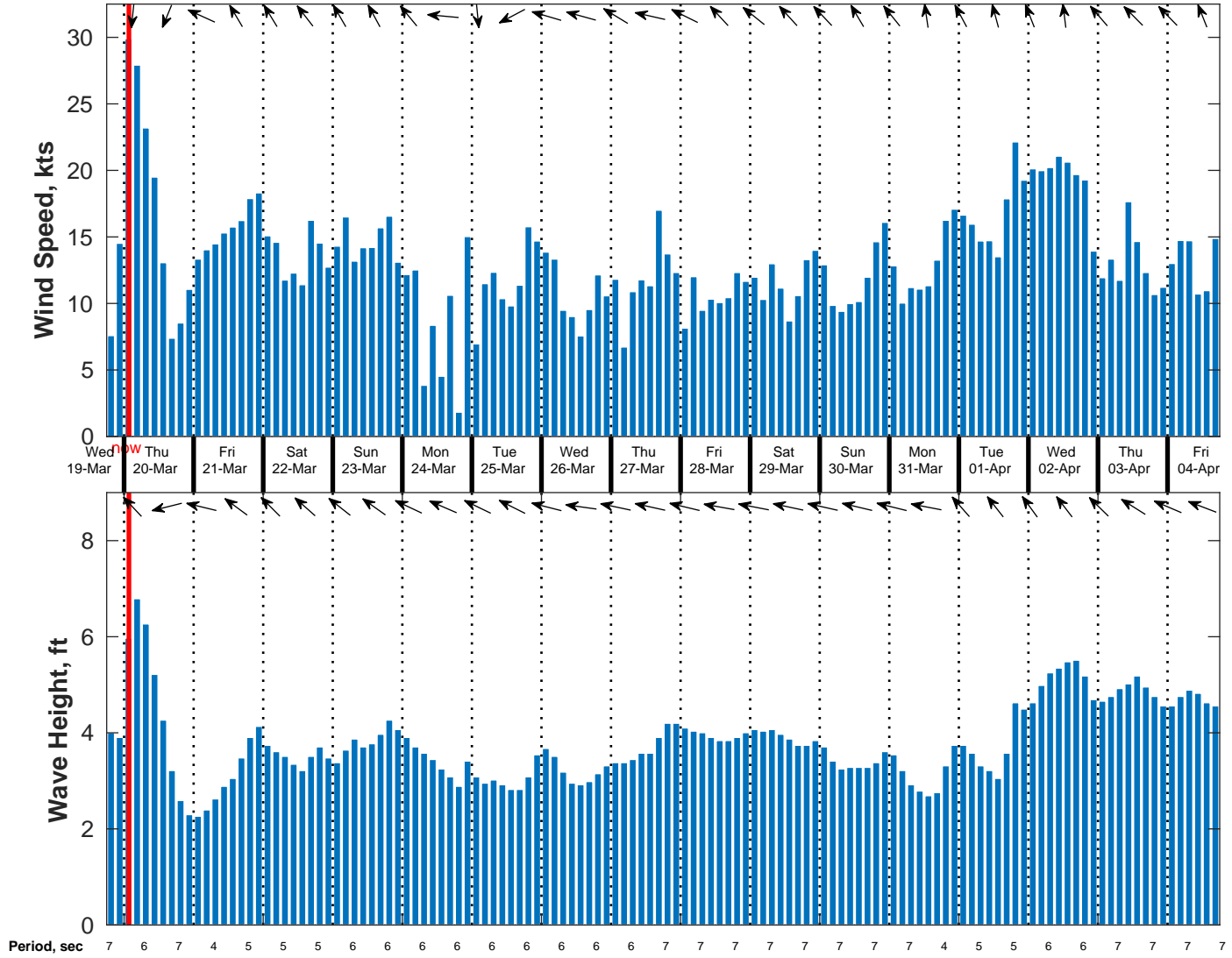
Wind & Wave Forecast for NDBC 42092 from 19-Mar-2025 18:00:00 to 04-Apr-2025 18:00:00
