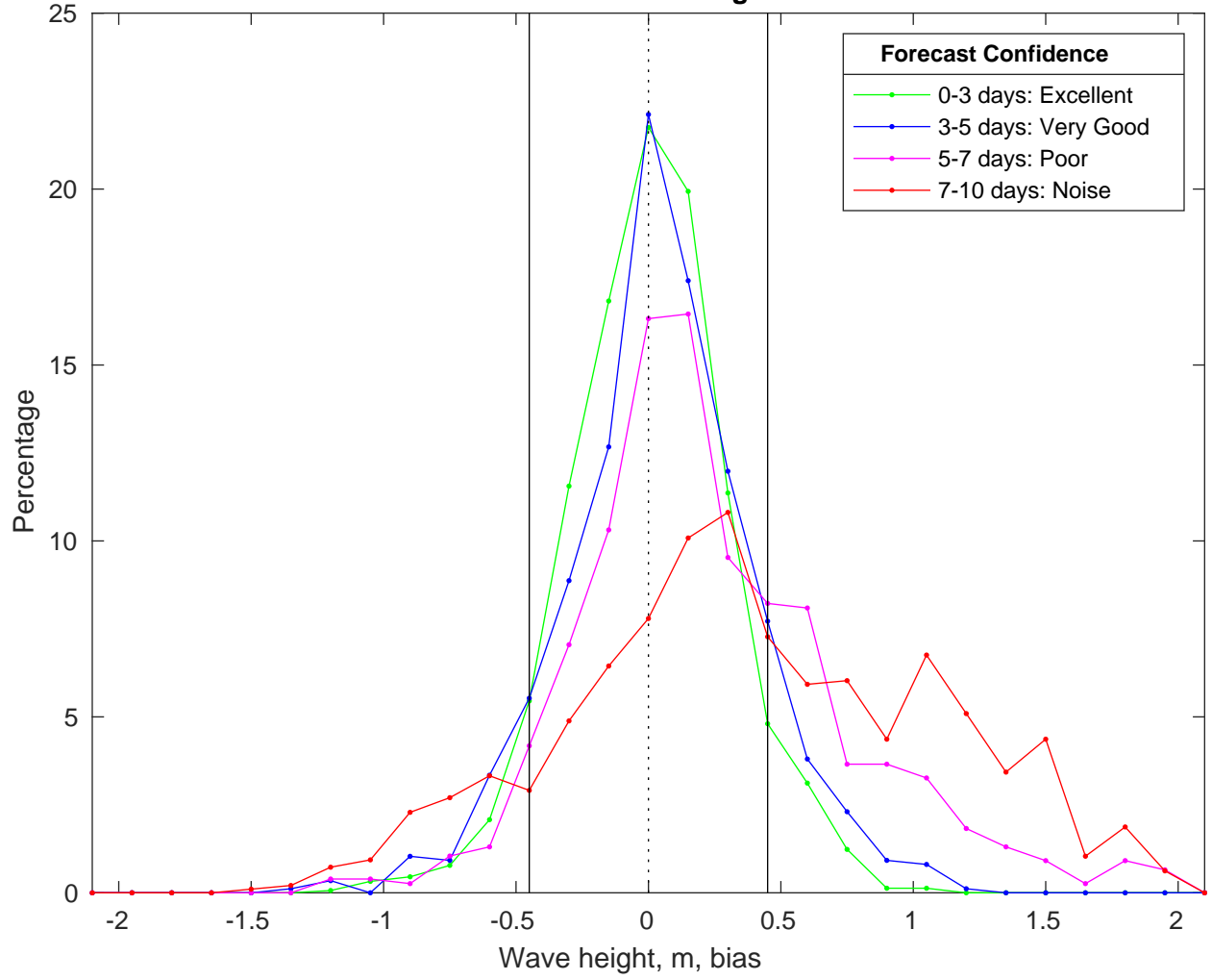
NDBC 46011 vs CMEMS Waves Bias Histogram: 20-Mar-2025
