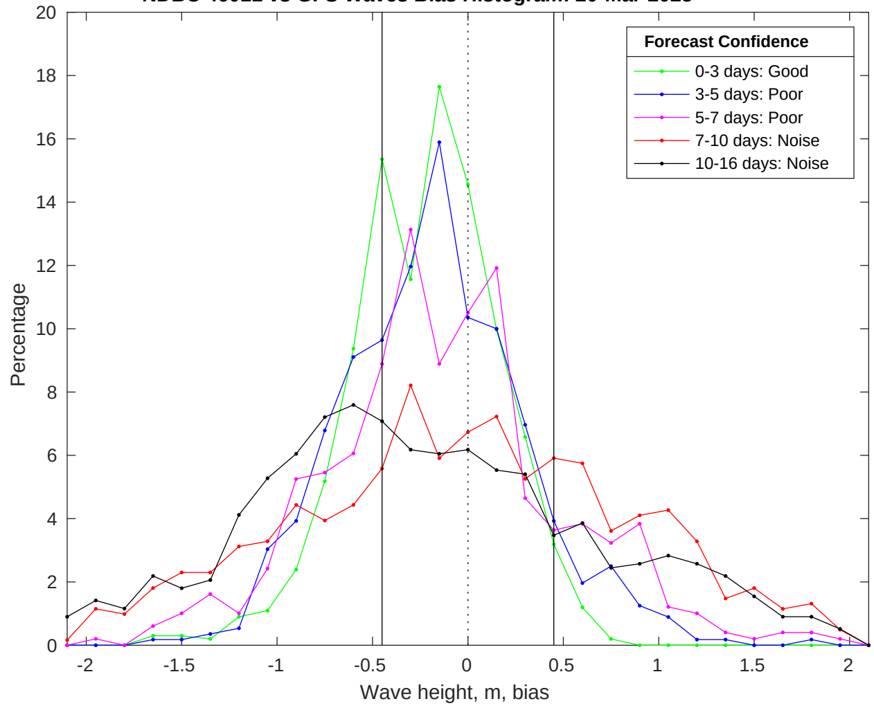
NDBC 46011 vs GFS Waves Bias Histogram: 20-Mar-2025
