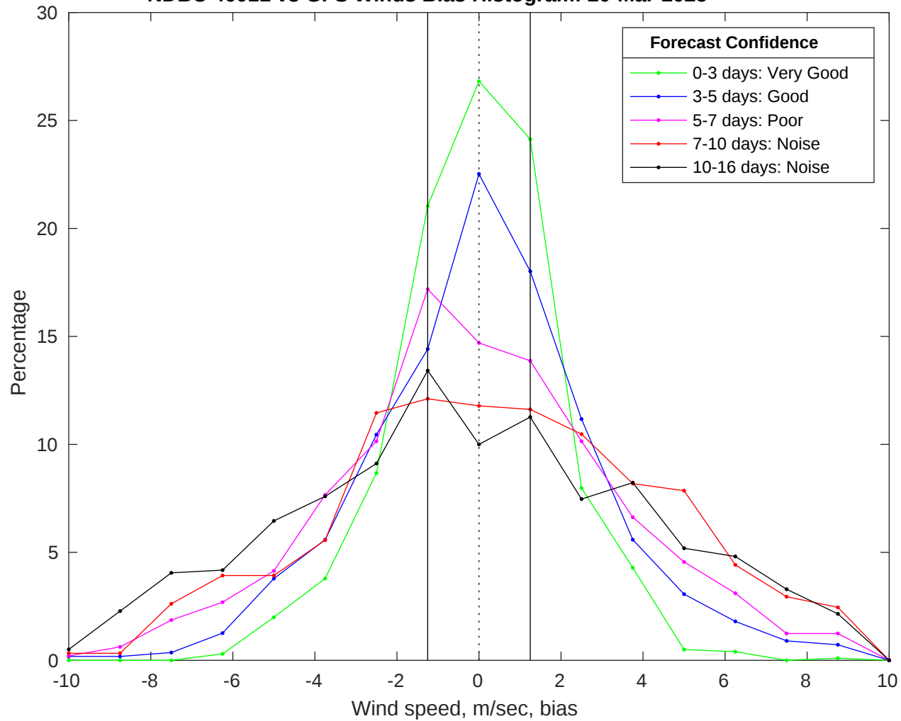
NDBC 46011 vs GFS Winds Bias Histogram: 20-Mar-2025
