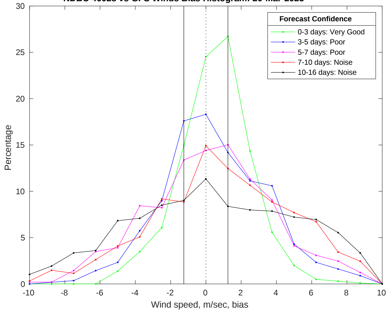
NDBC 46028 vs GFS Winds Bias Histogram: 20-Mar-2025
