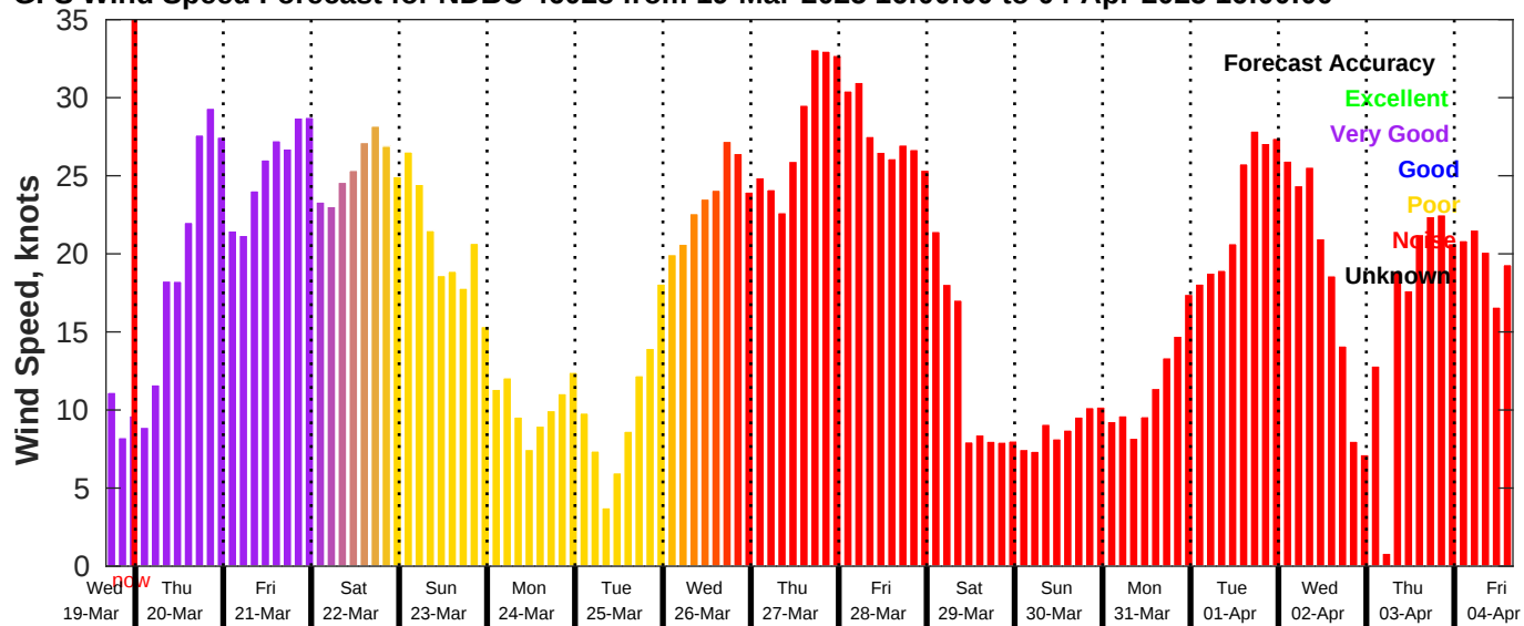
GFS Wind Speed Forecast for NDBC 46028 from 19-Mar-2025 16:00:00 to 04-Apr-2025 16:00:00
