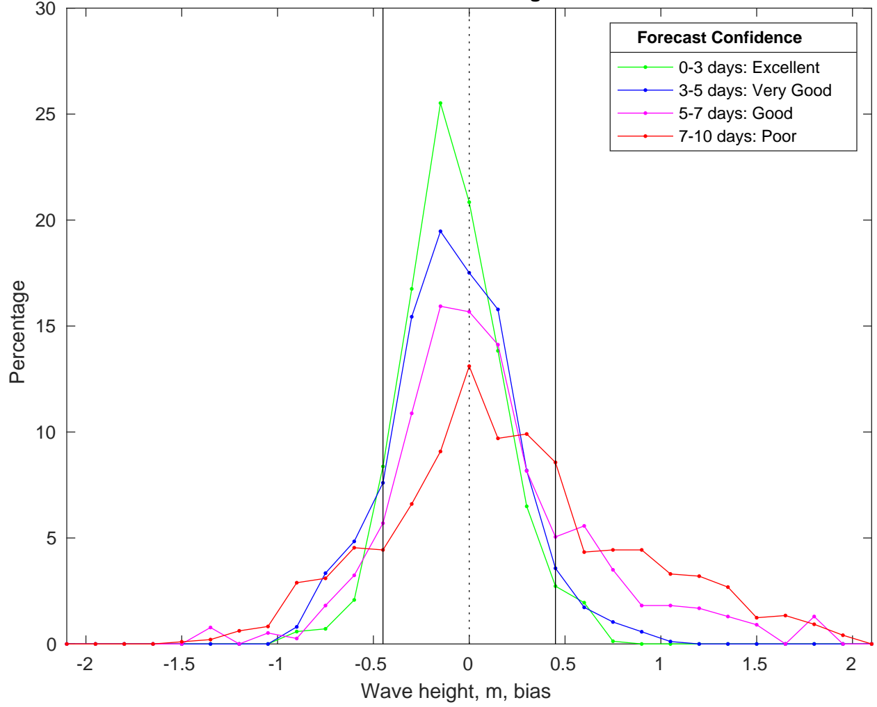
NDBC 46054 vs CMEMS Waves Bias Histogram: 20-Mar-2025
