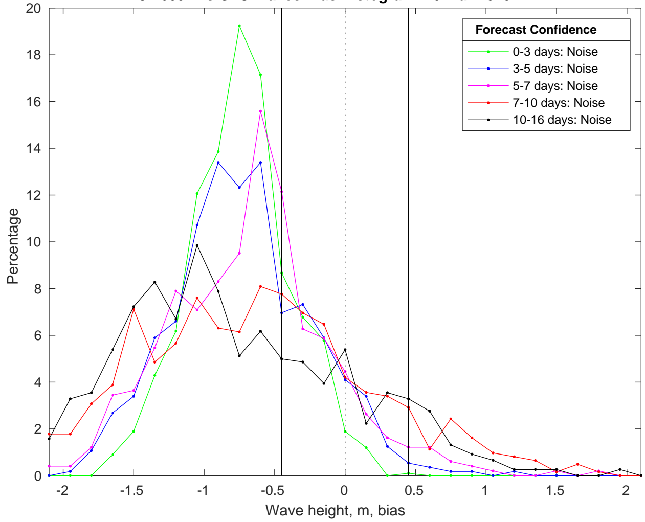
NDBC 46054 vs GFS Waves Bias Histogram: 20-Mar-2025
