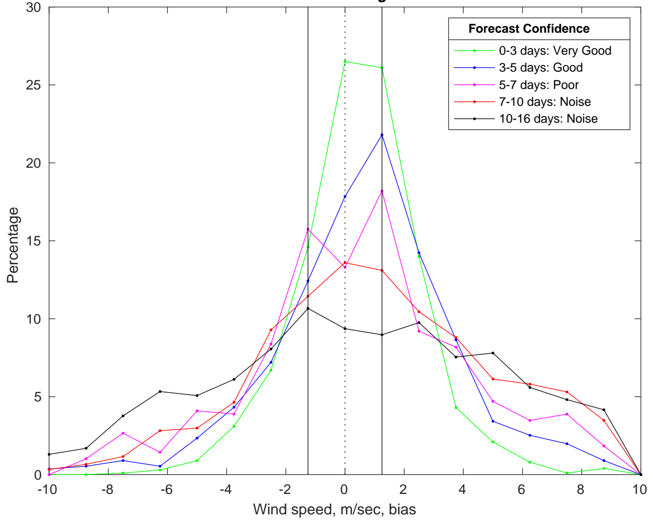
NDBC 46054 vs GFS Winds Bias Histogram: 20-Mar-2025
