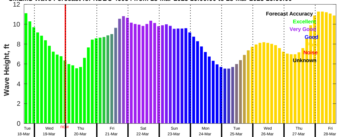
CMEMS Wave Forecast for NDBC 46054 from 18-Mar-2025 16:00:00 to 28-Mar-2025 16:00:00
