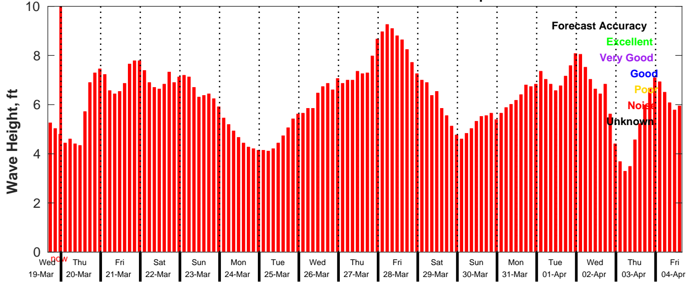
GFS Wave Forecast for NDBC 46054 from 19-Mar-2025 16:00:00 to 04-Apr-2025 16:00:00
