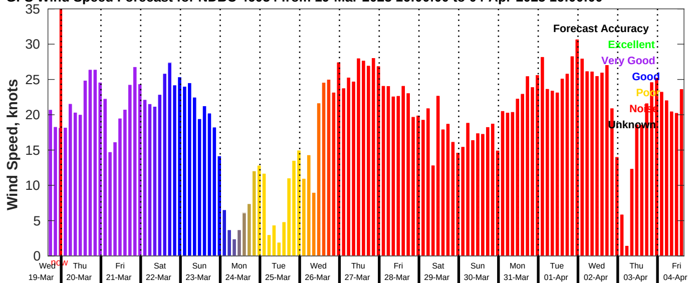
GFS Wind Speed Forecast for NDBC 46054 from 19-Mar-2025 16:00:00 to 04-Apr-2025 16:00:00
