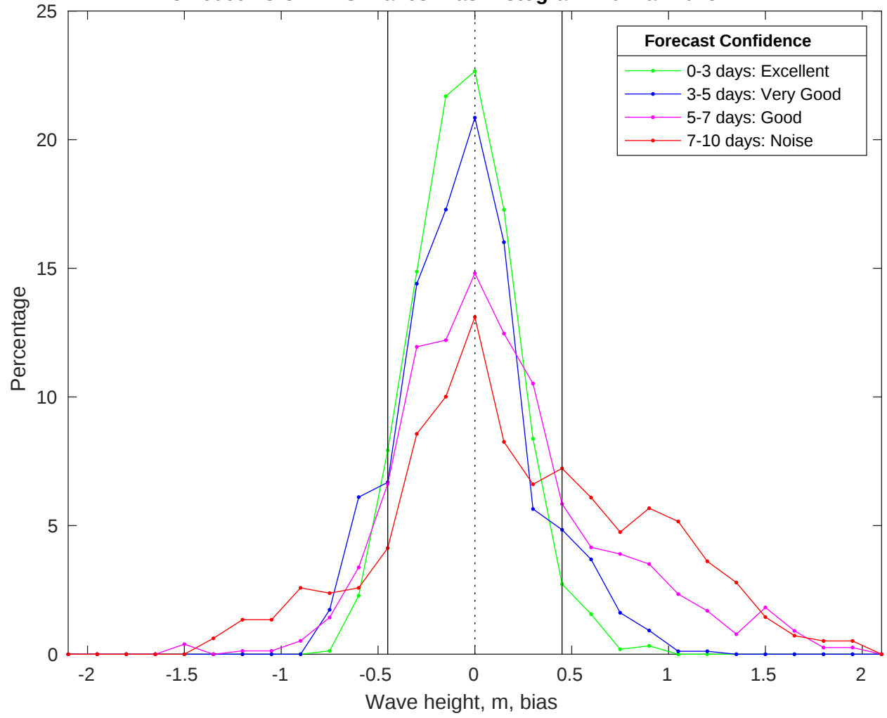
NDBC 46069 vs CMEMS Waves Bias Histogram: 20-Mar-2025
