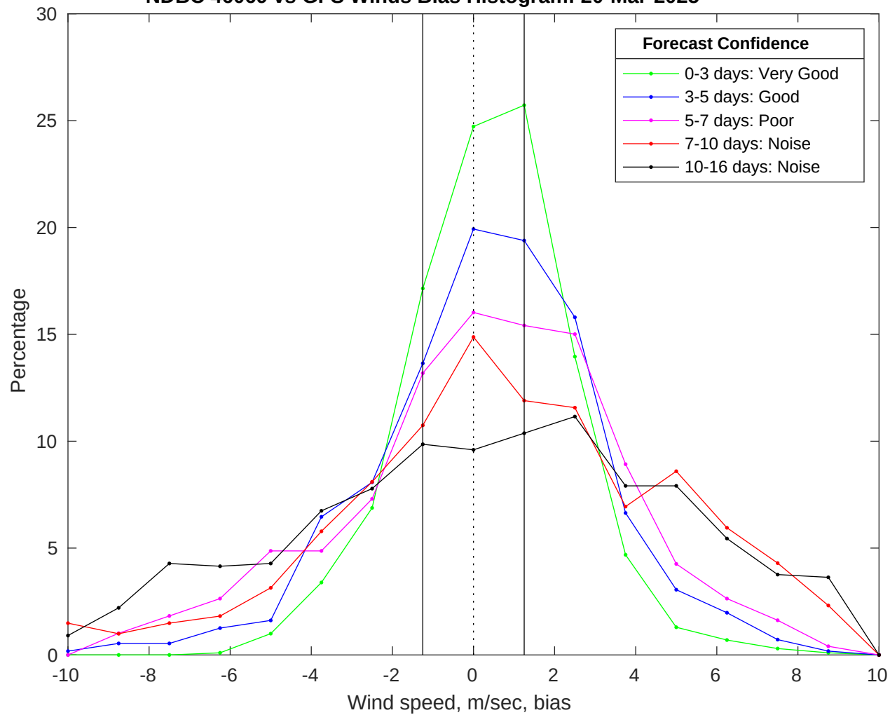
NDBC 46069 vs GFS Winds Bias Histogram: 20-Mar-2025
