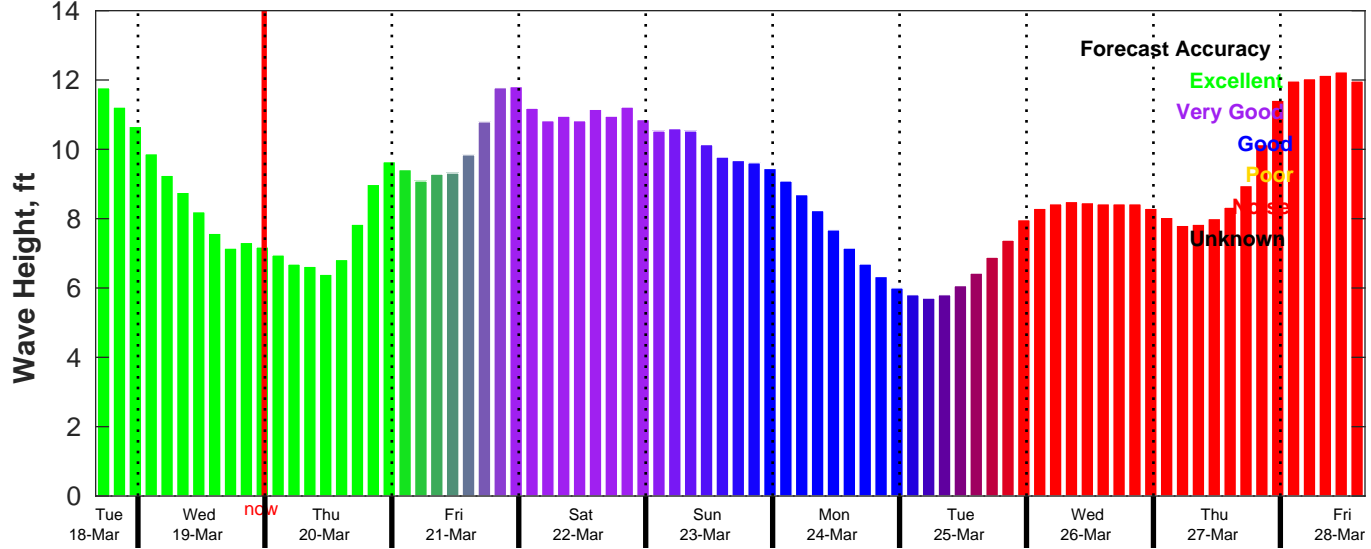
CMEMS Wave Forecast for NDBC 46069 from 18-Mar-2025 16:00:00 to 28-Mar-2025 16:00:00
