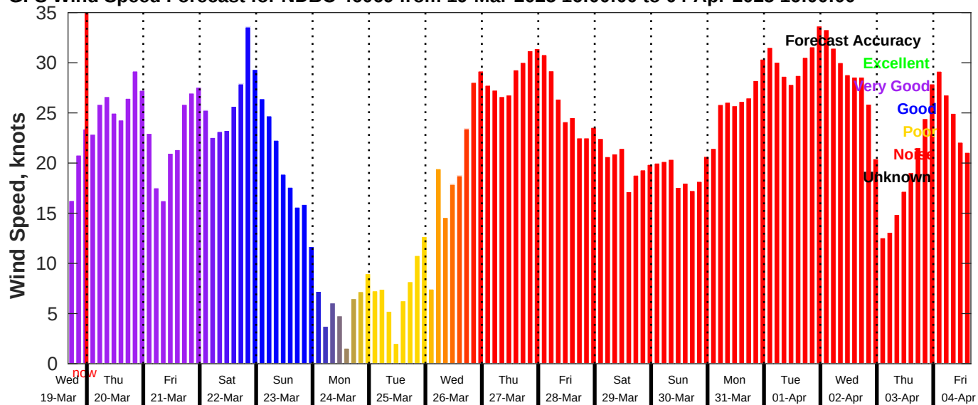
GFS Wind Speed Forecast for NDBC 46069 from 19-Mar-2025 16:00:00 to 04-Apr-2025 16:00:00
