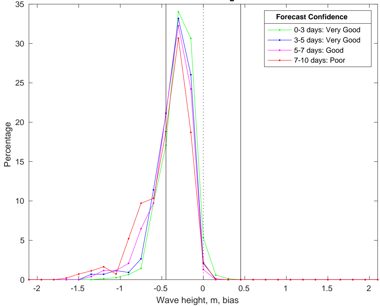
NDBC 51209 vs CMEMS Waves Bias Histogram: 20-Mar-2025
