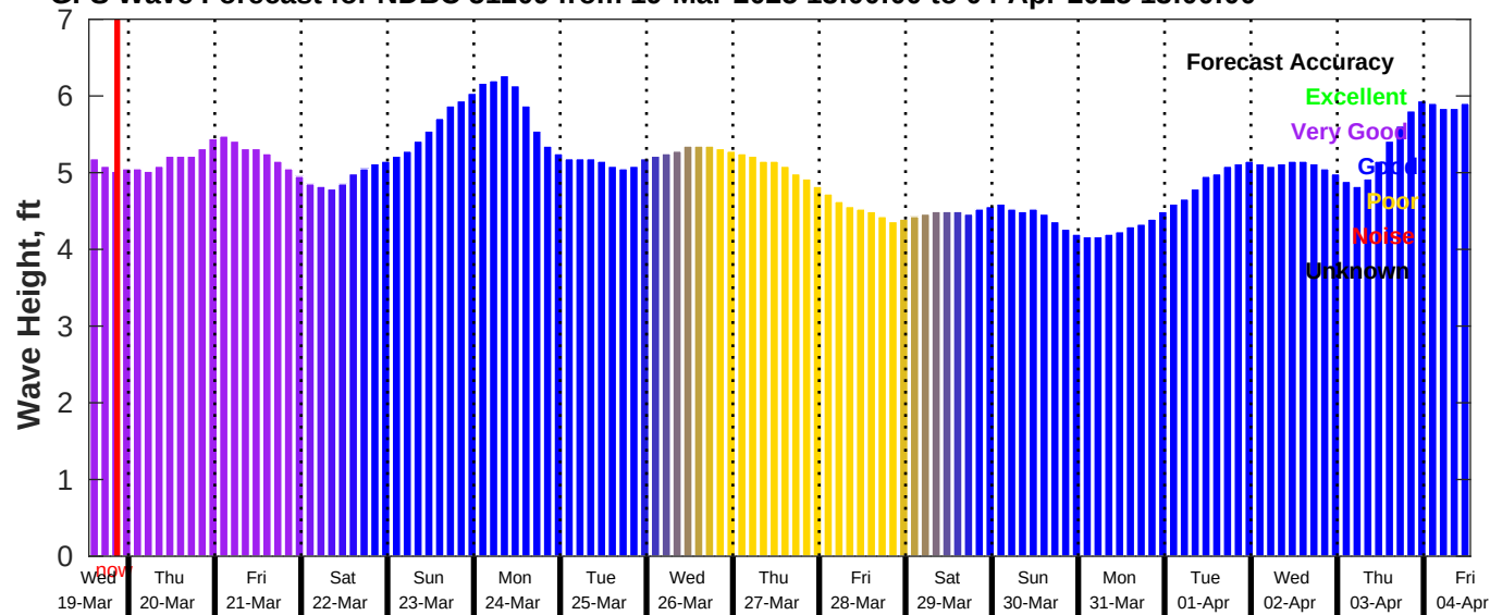
GFS Wave Forecast for NDBC 51209 from 19-Mar-2025 13:00:00 to 04-Apr-2025 13:00:00
