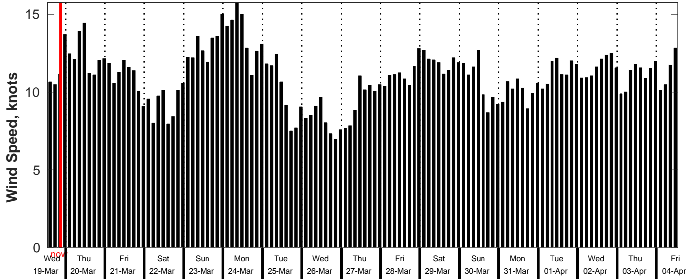
GFS Wind Speed Forecast for NDBC 51209 from 19-Mar-2025 13:00:00 to 04-Apr-2025 13:00:00
