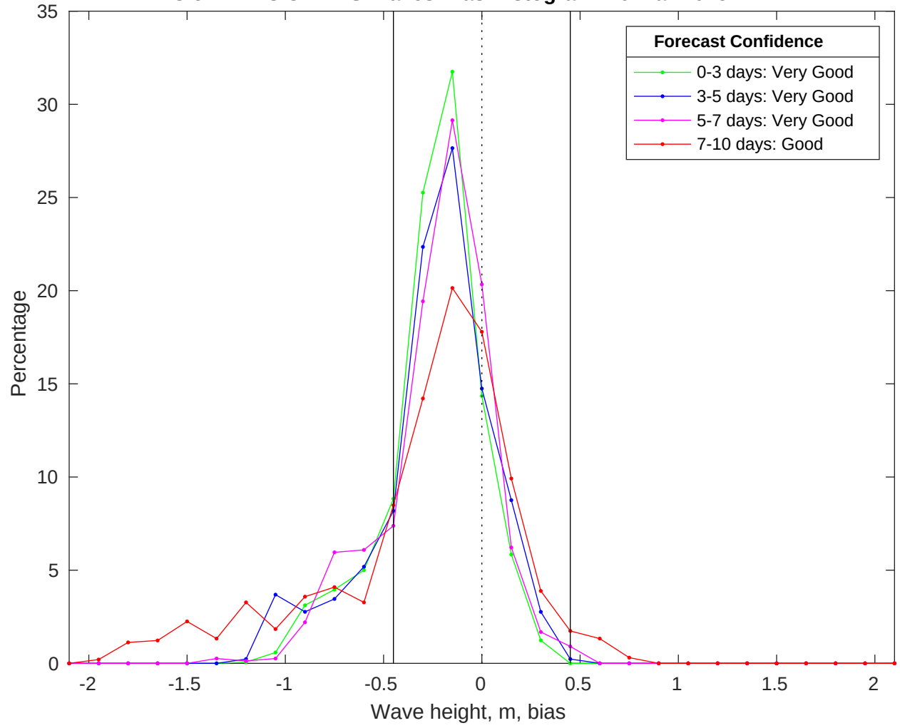
NDBC 52211 vs CMEMS Waves Bias Histogram: 20-Mar-2025
