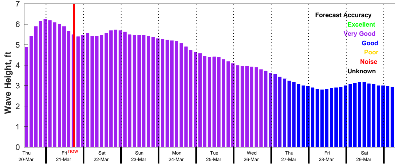
CMEMS Wave Forecast for NDBC 52211 from 19-Mar-2025 10:00:00 to 29-Mar-2025 10:00:00
