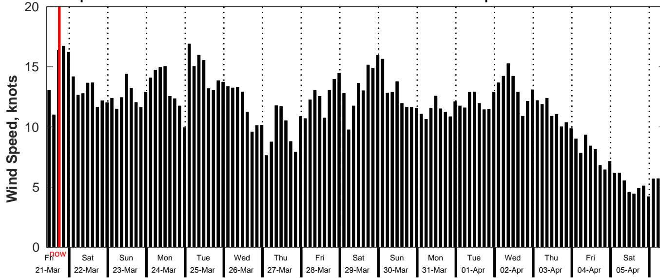
GFS Wind Speed Forecast for NDBC 52211 from 20-Mar-2025 10:00:00 to 05-Apr-2025 10:00:00
