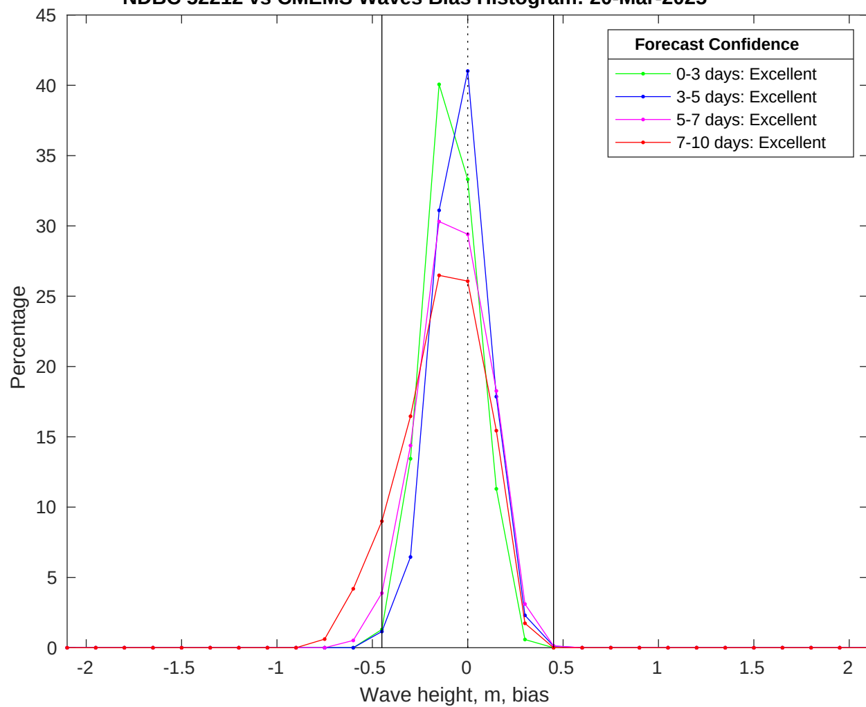
NDBC 52212 vs CMEMS Waves Bias Histogram: 20-Mar-2025
