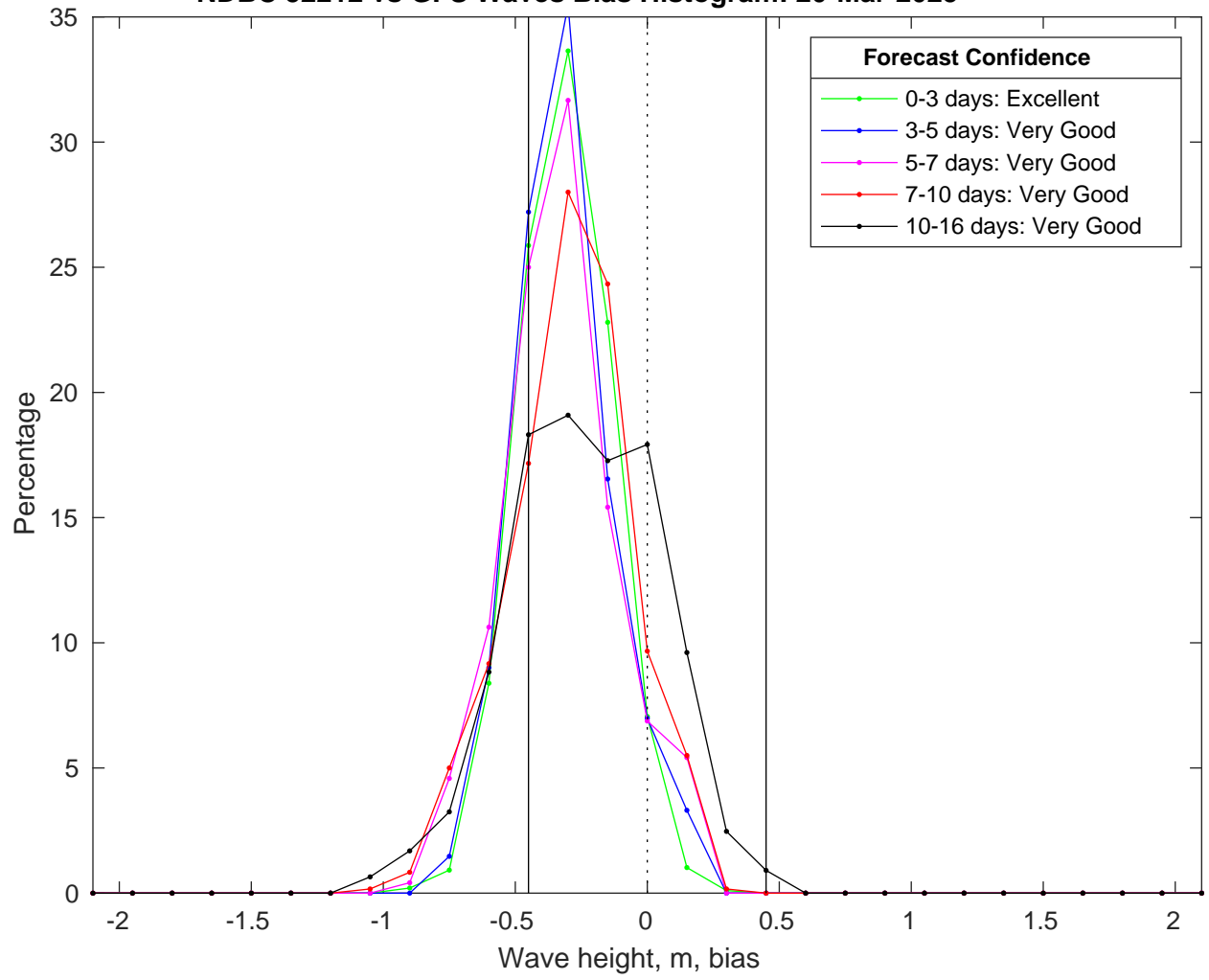
NDBC 52212 vs GFS Waves Bias Histogram: 20-Mar-2025
