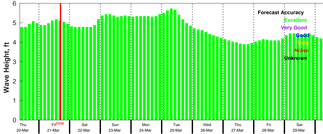
CMEMS Wave Forecast for NDBC 52212 from 19-Mar-2025 09:00:00 to 29-Mar-2025 09:00:00
