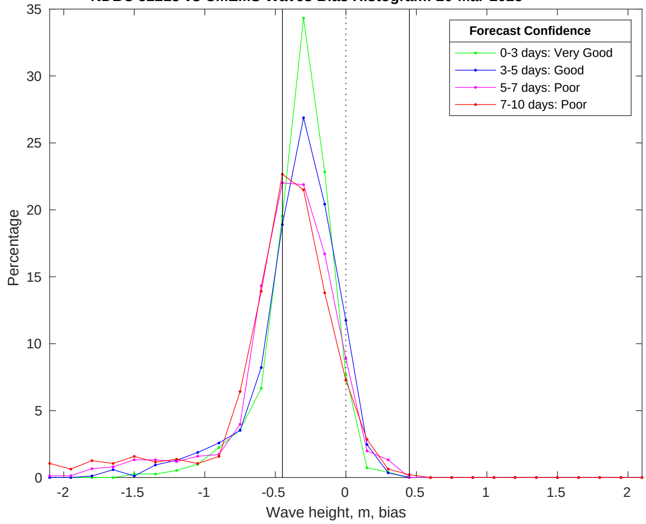
NDBC 52213 vs CMEMS Waves Bias Histogram: 20-Mar-2025
