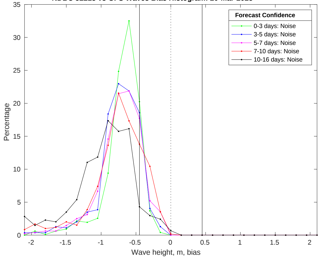
NDBC 52213 vs GFS Waves Bias Histogram: 20-Mar-2025
