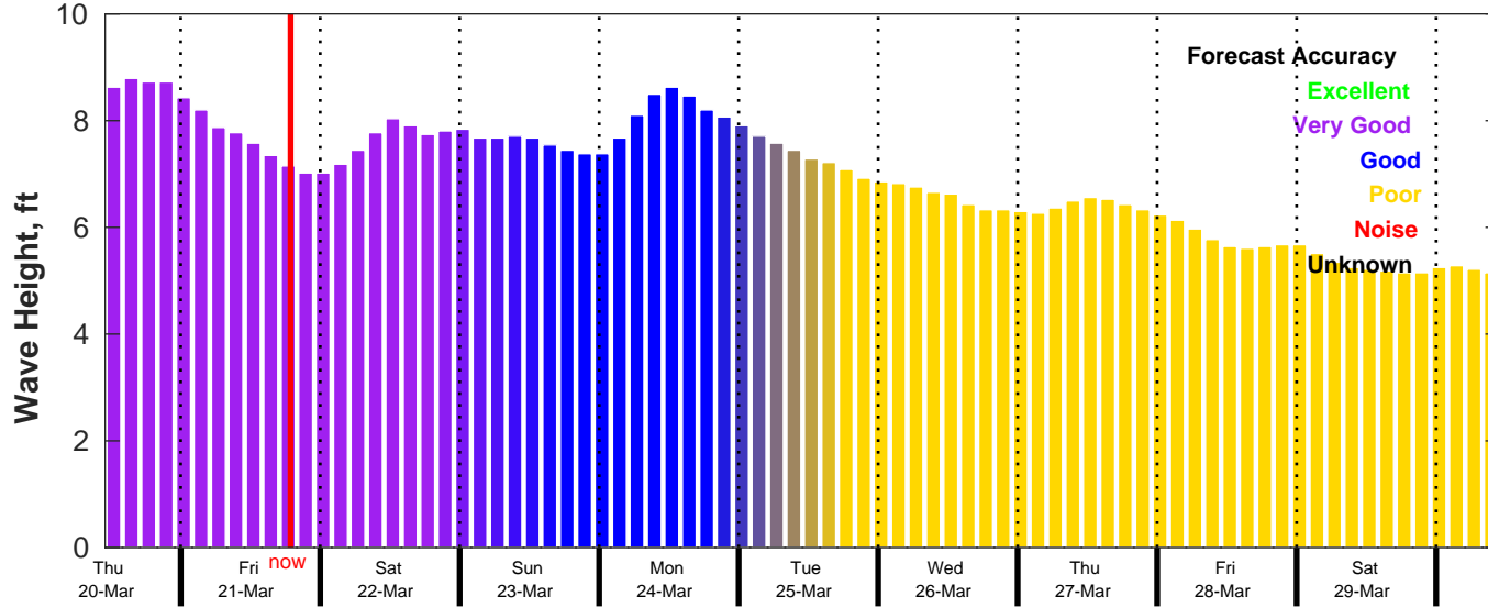
CMEMS Wave Forecast for NDBC 52213 from 19-Mar-2025 11:00:00 to 29-Mar-2025 11:00:00
