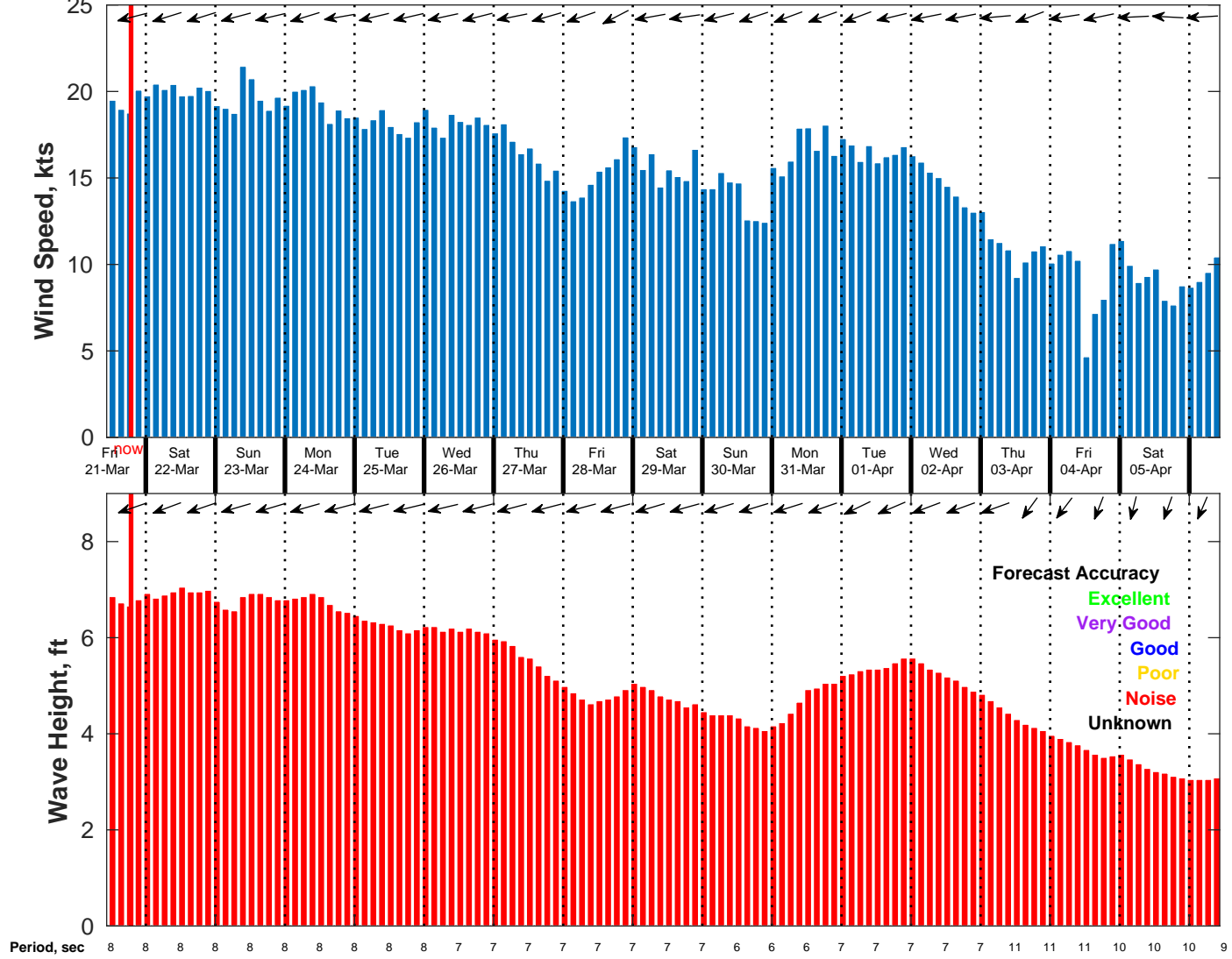
Wind & Wave Forecast for NDBC 52213 from 20-Mar-2025 11:00:00 to 05-Apr-2025 11:00:00
