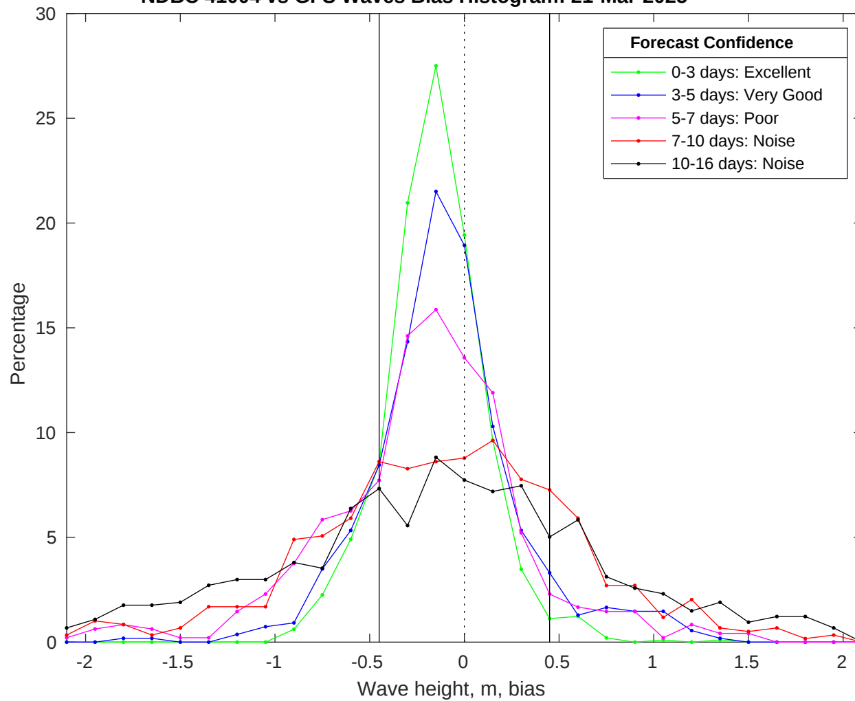
NDBC 41004 vs GFS Waves Bias Histogram: 21-Mar-2025
