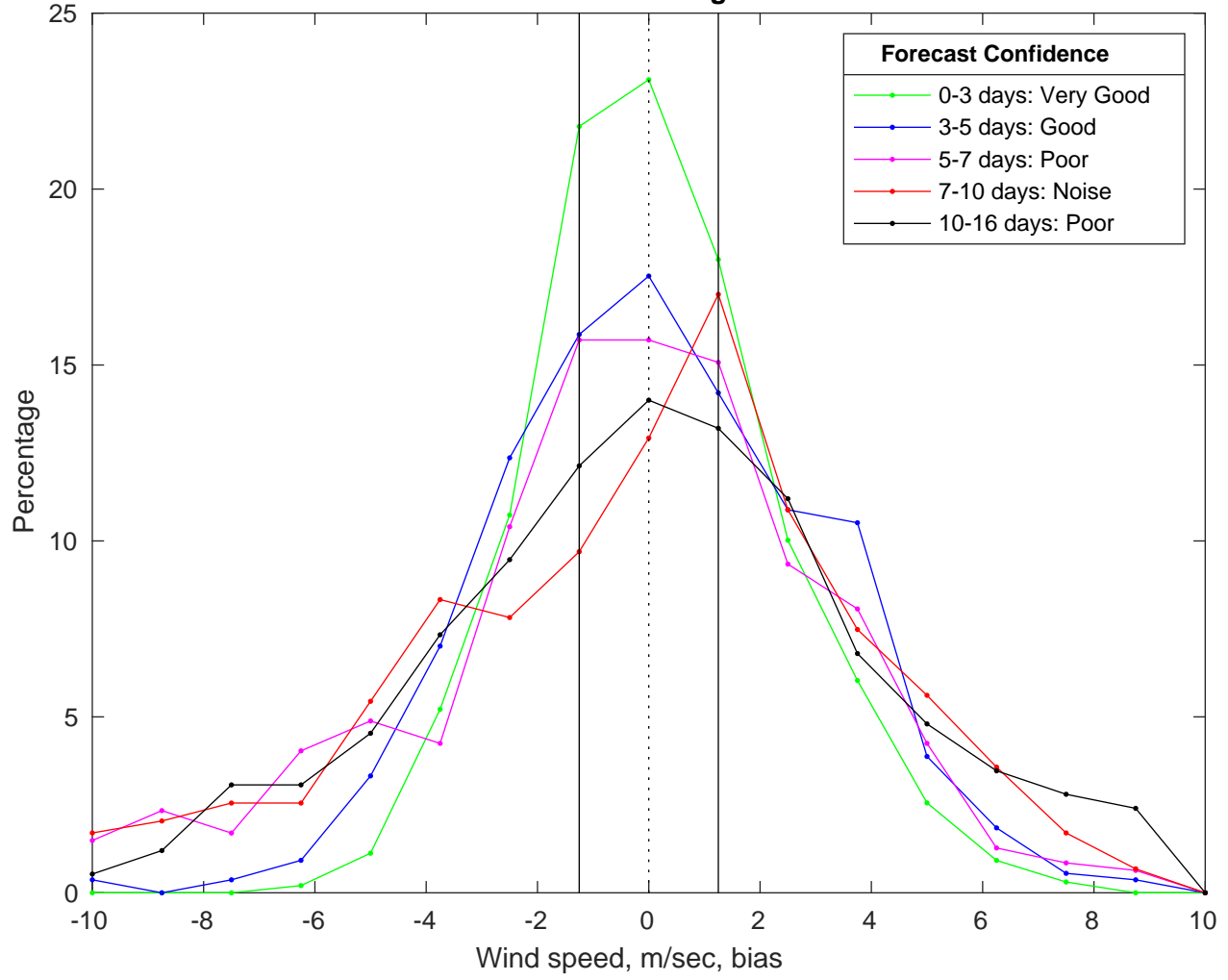
NDBC 41004 vs GFS Winds Bias Histogram: 21-Mar-2025
