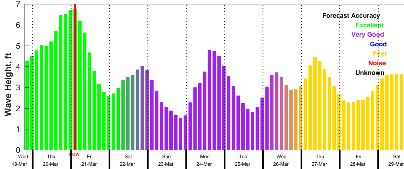
CMEMS Wave Forecast for NDBC 41004 from 19-Mar-2025 19:00:00 to 29-Mar-2025 19:00:00
