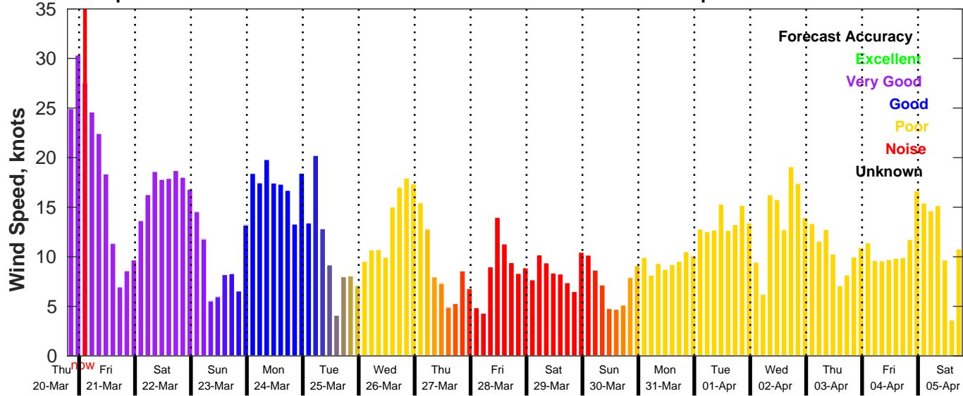
GFS Wind Speed Forecast for NDBC 41004 from 20-Mar-2025 19:00:00 to 05-Apr-2025 19:00:00
