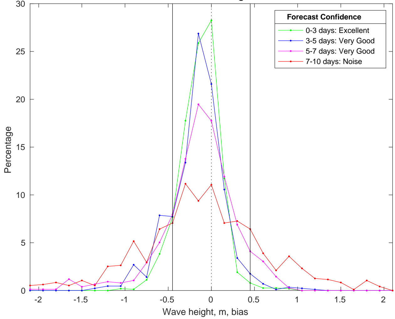
NDBC 41013 vs CMEMS Waves Bias Histogram: 21-Mar-2025
