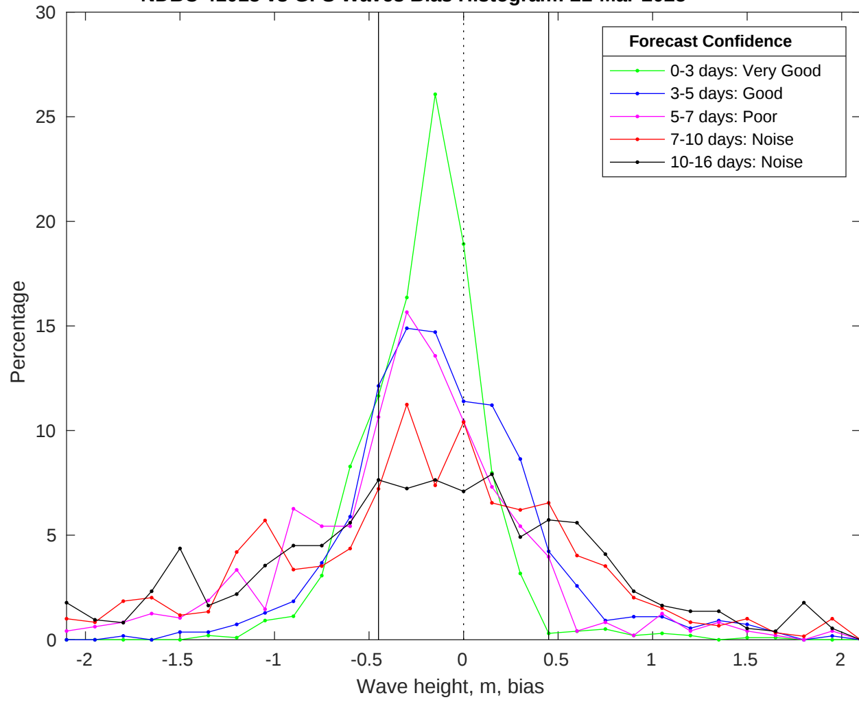
NDBC 41013 vs GFS Waves Bias Histogram: 21-Mar-2025
