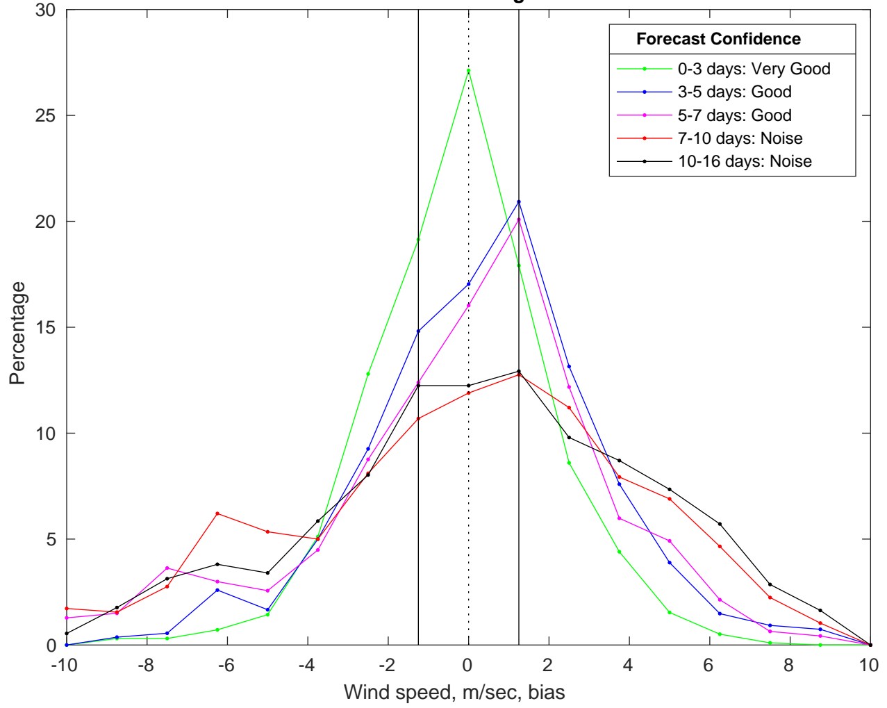
NDBC 41013 vs GFS Winds Bias Histogram: 21-Mar-2025
