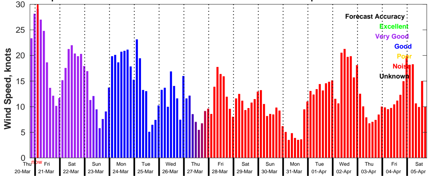
GFS Wind Speed Forecast for NDBC 41013 from 20-Mar-2025 19:00:00 to 05-Apr-2025 19:00:00
