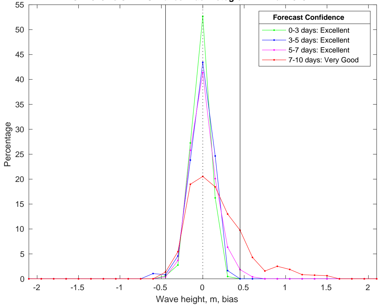
NDBC 41040 vs CMEMS Waves Bias Histogram: 21-Mar-2025
