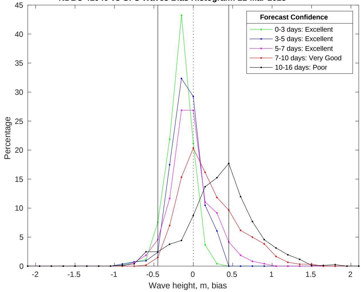
NDBC 41040 vs GFS Waves Bias Histogram: 21-Mar-2025
