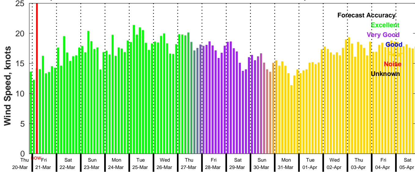
GFS Wind Speed Forecast for NDBC 41040 from 20-Mar-2025 21:00:00 to 05-Apr-2025 21:00:00
