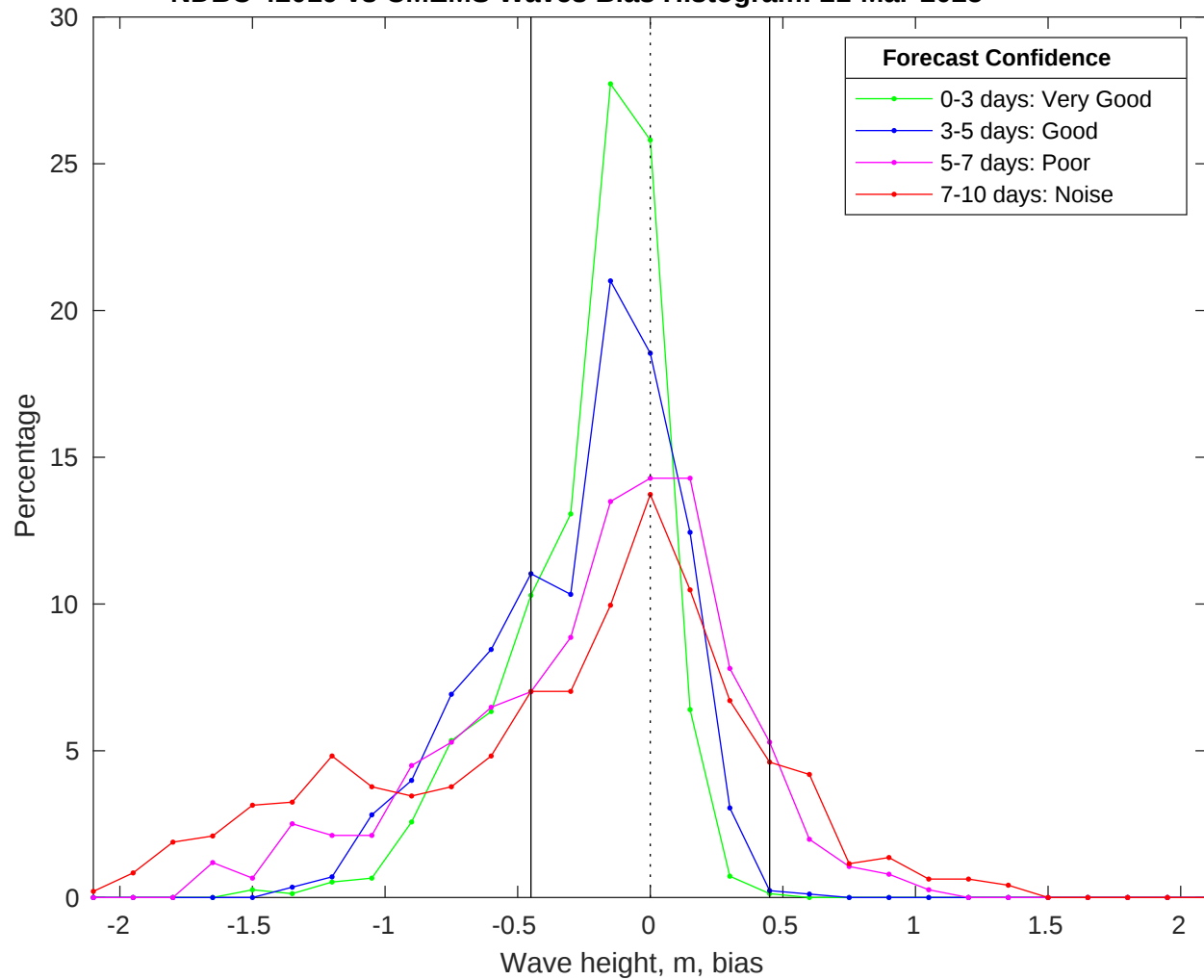
NDBC 42019 vs CMEMS Waves Bias Histogram: 21-Mar-2025
