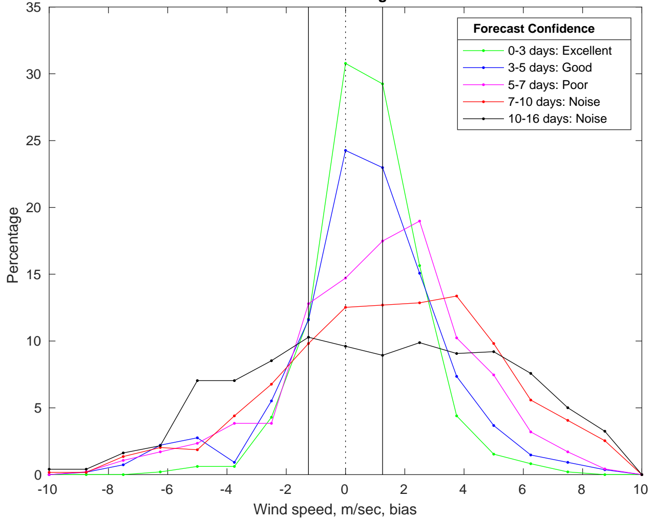
NDBC 42019 vs GFS Winds Bias Histogram: 21-Mar-2025
