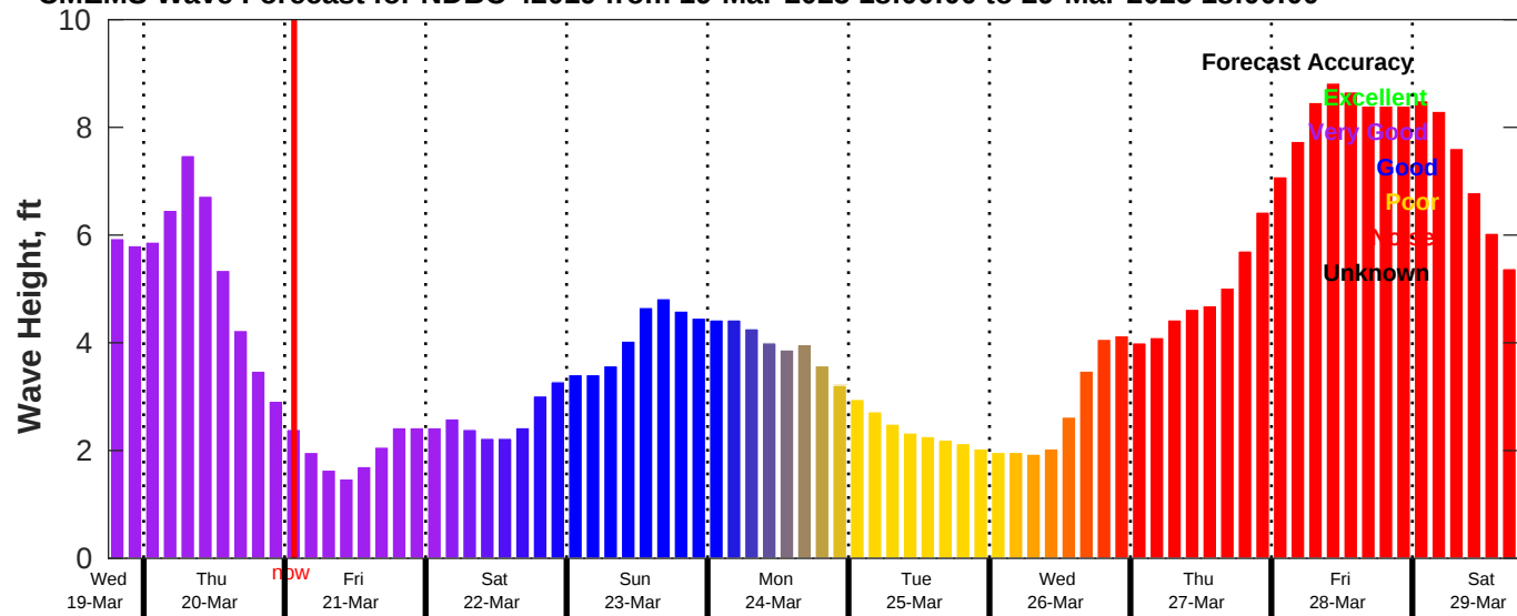
CMEMS Wave Forecast for NDBC 42019 from 19-Mar-2025 18:00:00 to 29-Mar-2025 18:00:00
